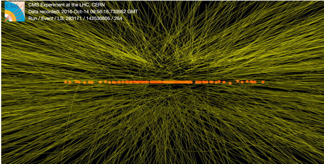
Figure 2.3: Collisions recorded by the CMS detector on October 14 2016 during the high pileup fill [76]. The events are from isolated bunches with an average pileup of roughly 100.
