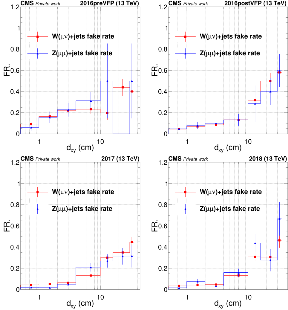
Figure 6.11: The values of f_W and f_{DY} measured in 2016 pre-VFP, 2016 post-VFP, 2017 and 2018 data-taking periods, as a function of jet d_{xy} .
