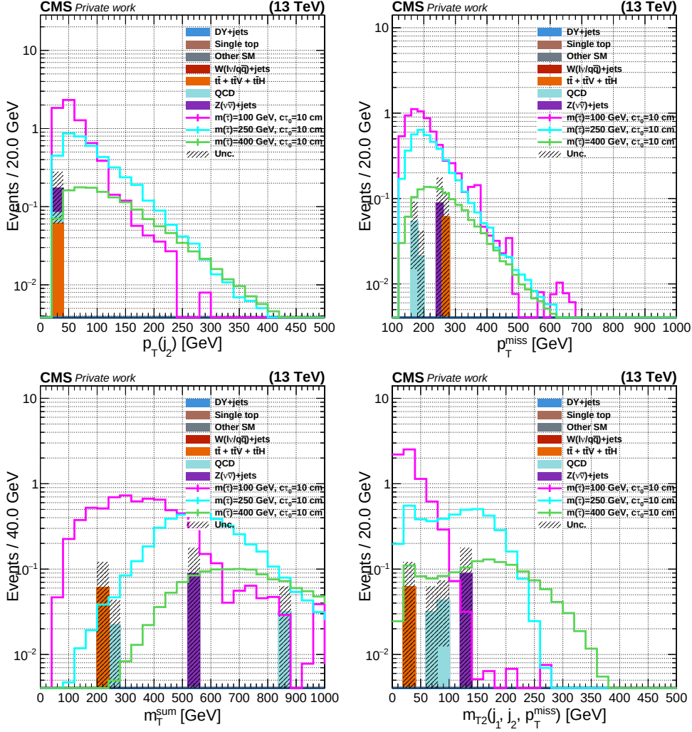
Figure 6.7: Distributions of p_T^{j2} , p_T^{miss} , \Sigma m_T and m_{T2} in BRT2, showing the contributions from different SM processes.
