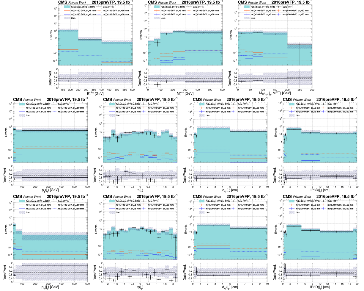
Figure A.5: From left to right and top to bottom: the distributions of p_T^{\text{miss}} , \Sigma m_T , m_{T2} , p_T^{j1} , \eta^{j1} , d_{xy}^{j1} , \text{IP3D}^{j1} , p_T^{j2} , \eta^{j2} , d_{xy}^{j2} , \text{IP3D}^{j2} , showing the background prediction in BRT1 from BRT0. The prediction uses f_W(p_T, d_{xy}) , and the plots correspond to the 2016 pre-VFP data-taking period.
