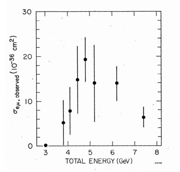
Figure 4.1: The observed cross-section for the signature of e\mu events [117]. The first observation of \tau lepton.
