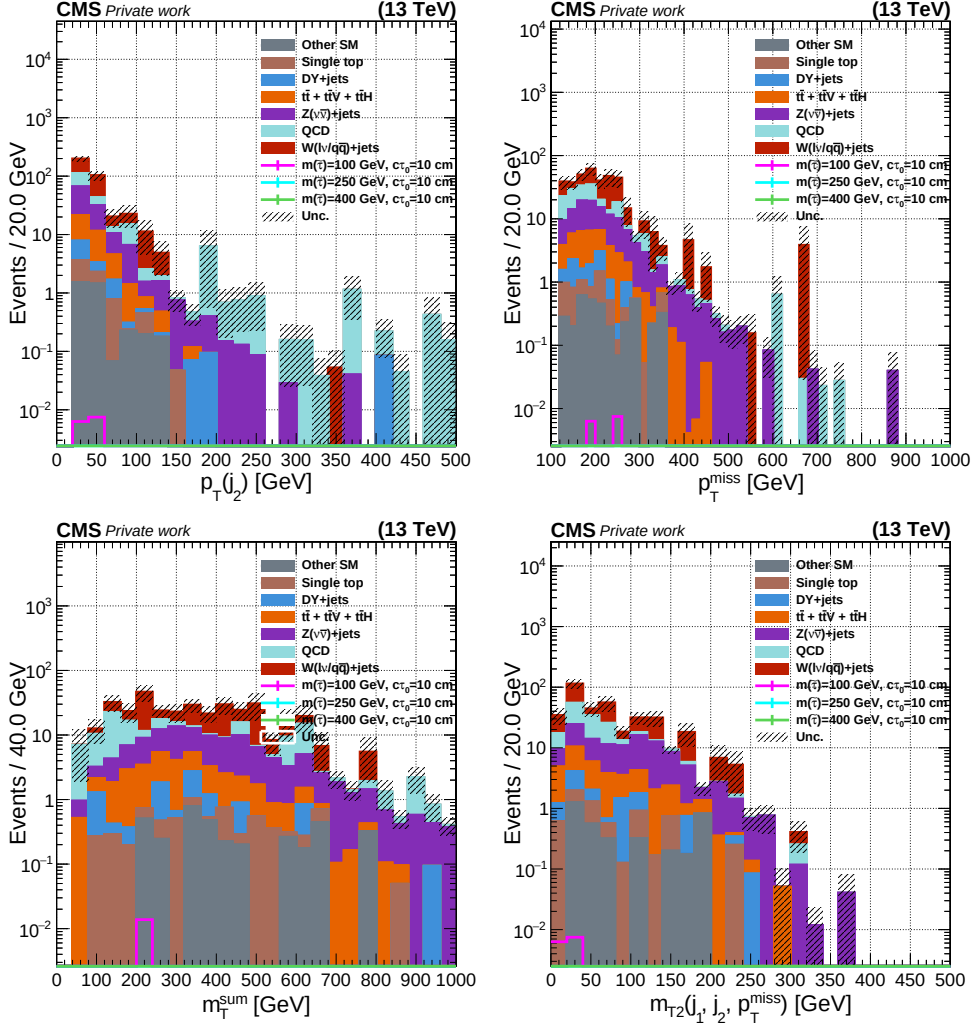
Figure 6.5: Distributions of p_T^{j2} , p_T^{\text{miss}} , \Sigma m_T and m_{T2} in BRT0, showing the contributions from different SM processes.
