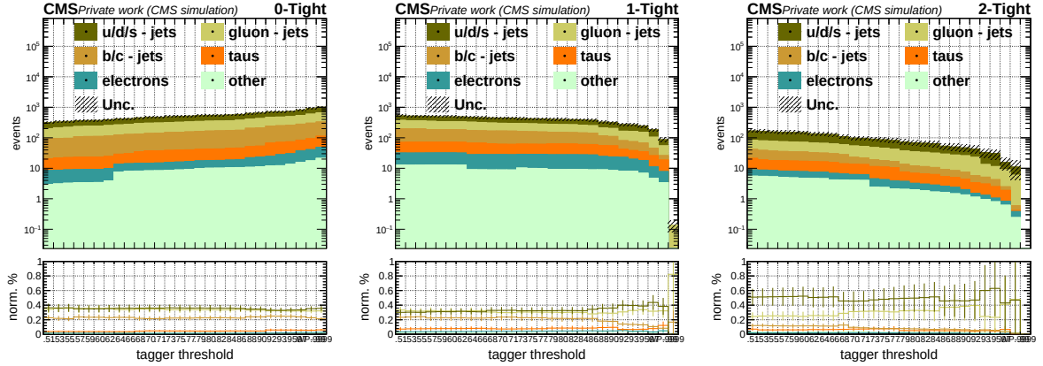
Figure 6.13: Absolute and relative contribution from jets of different flavours as a function of the DisTau score threshold starting from 0.5 and up to 0.999, in BRT0 (left), BRT1 (central), and BRT2 (right).
