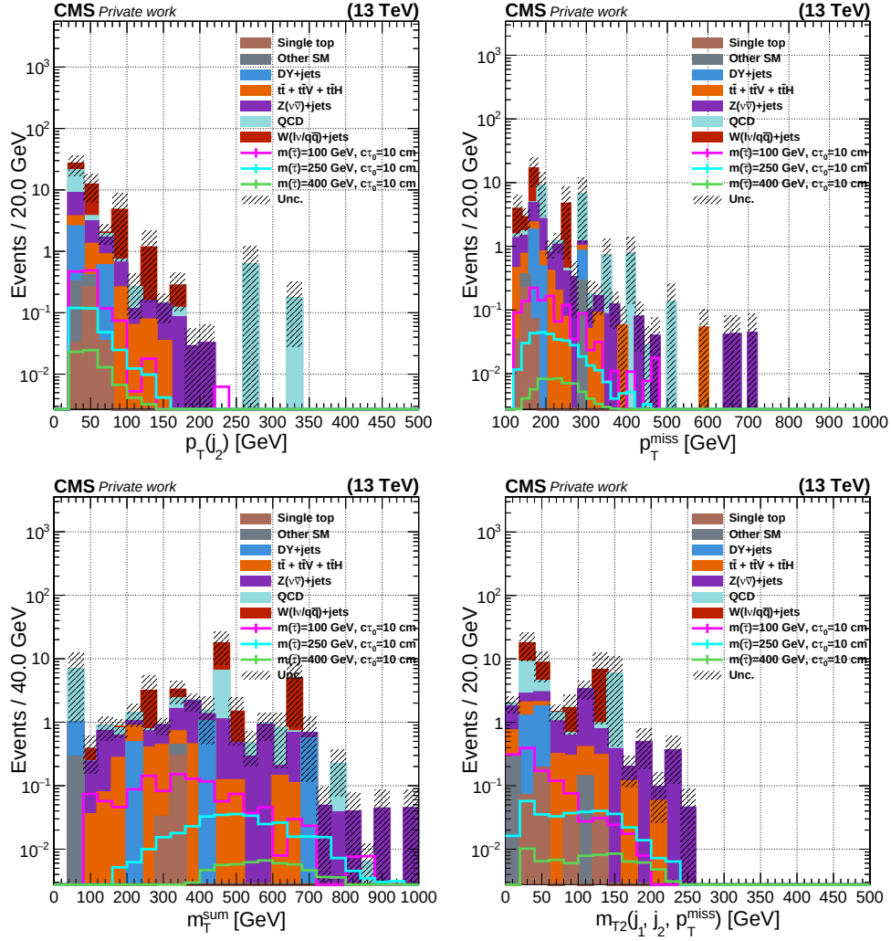
Figure 6.6: Distributions of p_T^{j2} , p_T^{miss} , \Sigma m_T and m_{T2} in BRT1, showing the contributions from different SM processes.
