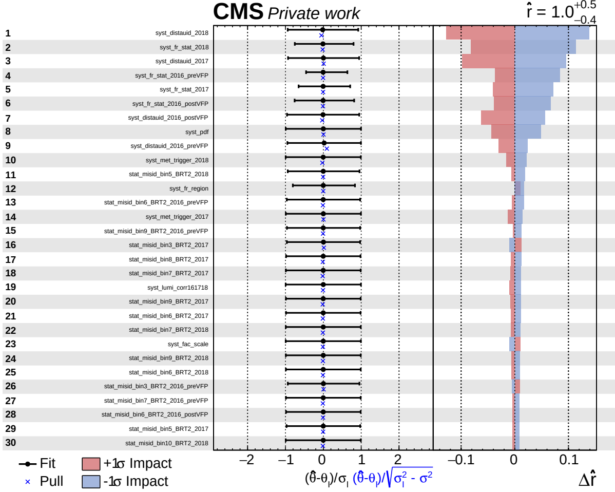
Figure 6.24: The most relevant 30 uncertainties, sorted by the impact and associated pulls for the \tilde{\tau} mass equal to 200 GeV and c\tau_0 = 100 mm, derived from a signal plus background Asimov dataset. The middle panel illustrates the pulls, while the right panel depicts the impact on the signal strength when scaling the uncertainty by 1\sigma upward (red band) and downward (blue band).
