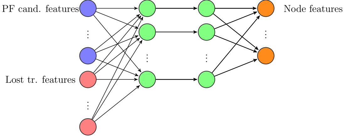
Figure 5.8: Illustrative diagram of node feature pre-processing.
